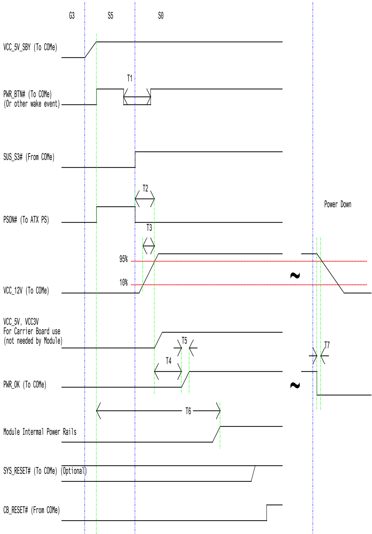
Figure 21: ATX Style Power Up Boot – Controlled by Power Button
