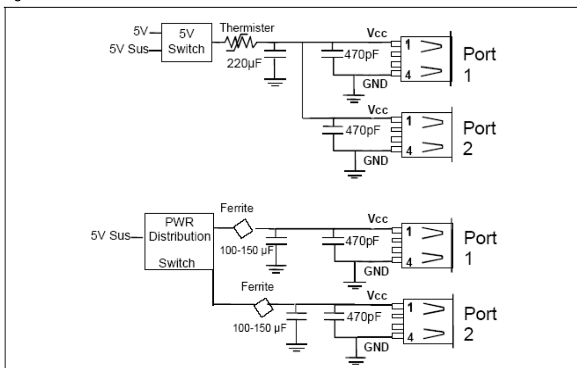
Figure 9: USB 2.0 Good Downstream Power Connection
