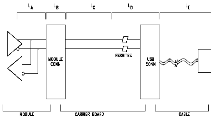
Figure 8: USB Insertion Loss Budget
