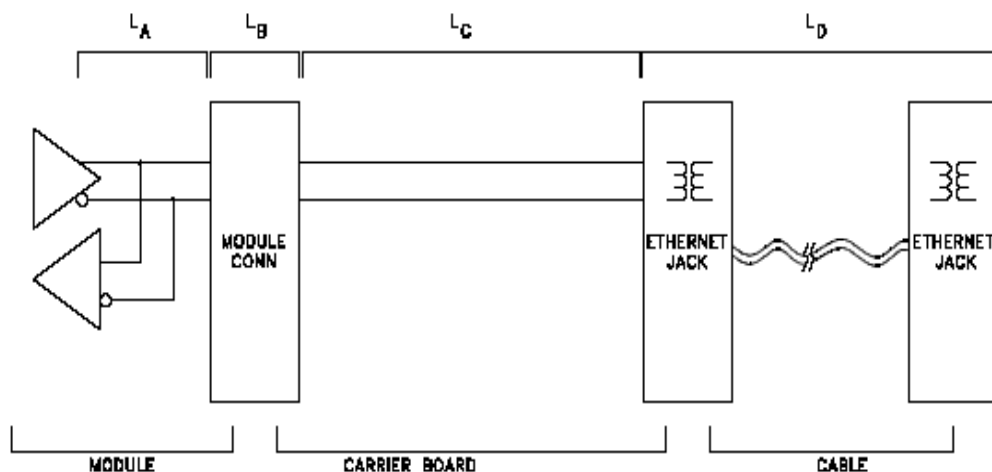
Figure 6: 10/100/1000 Ethernet Insertion Loss Budget
