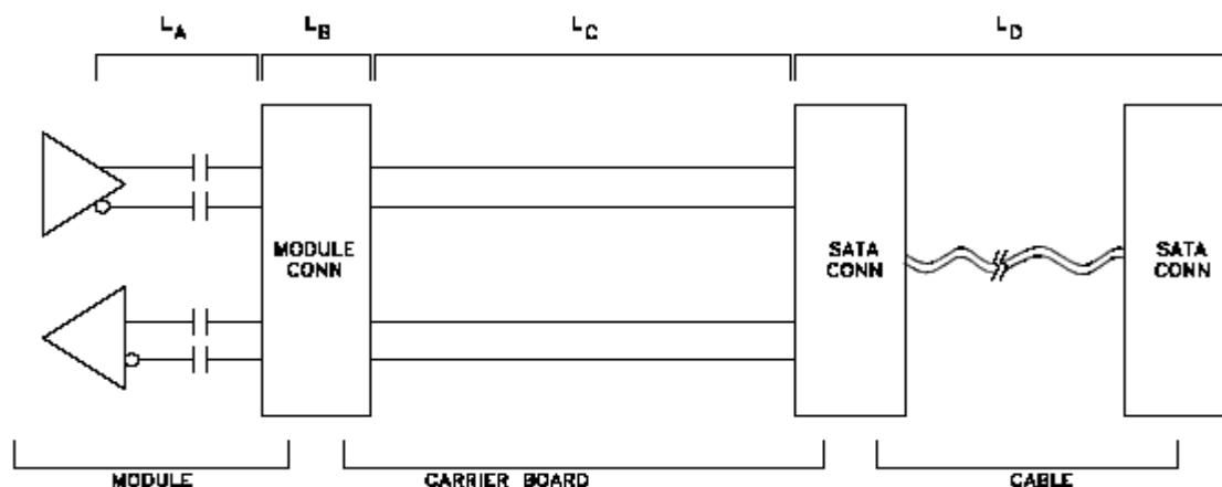
Figure 14: SATA Insertion Loss Budget
