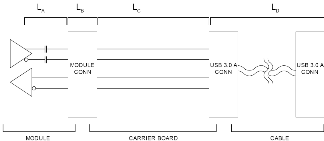
Figure 12: USB3.0 Insertion Loss Budget
