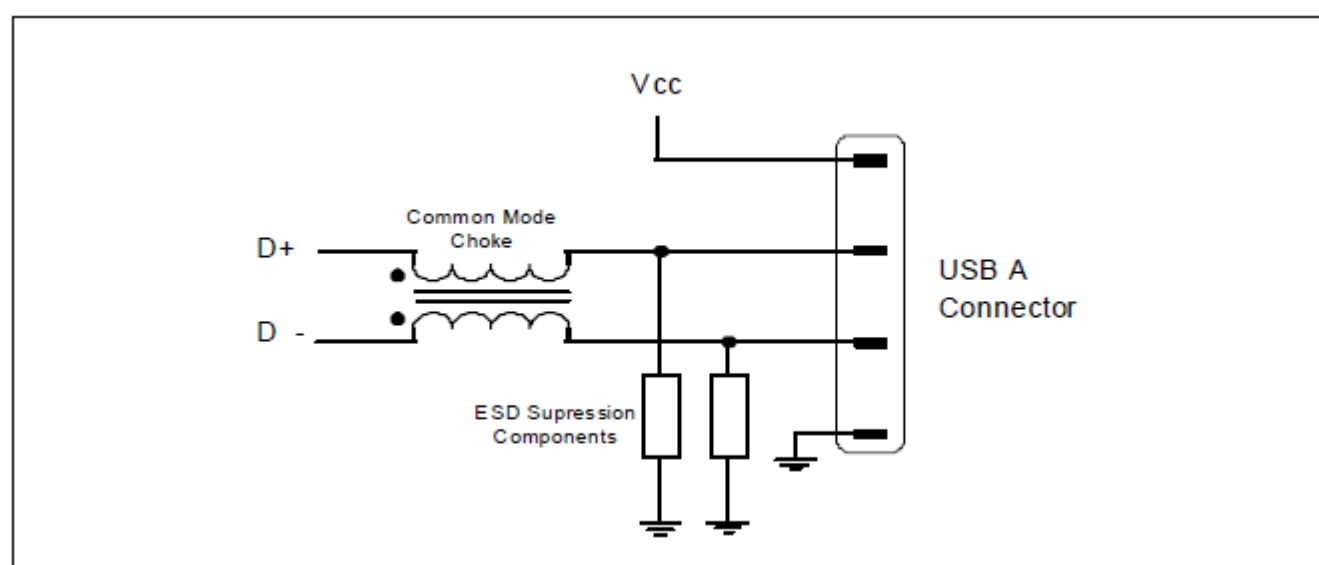
Figure 10: USB 2.0 A Common Mode Choke
