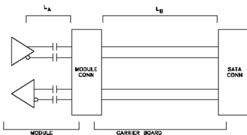
Figure 15: Topology for SATA
