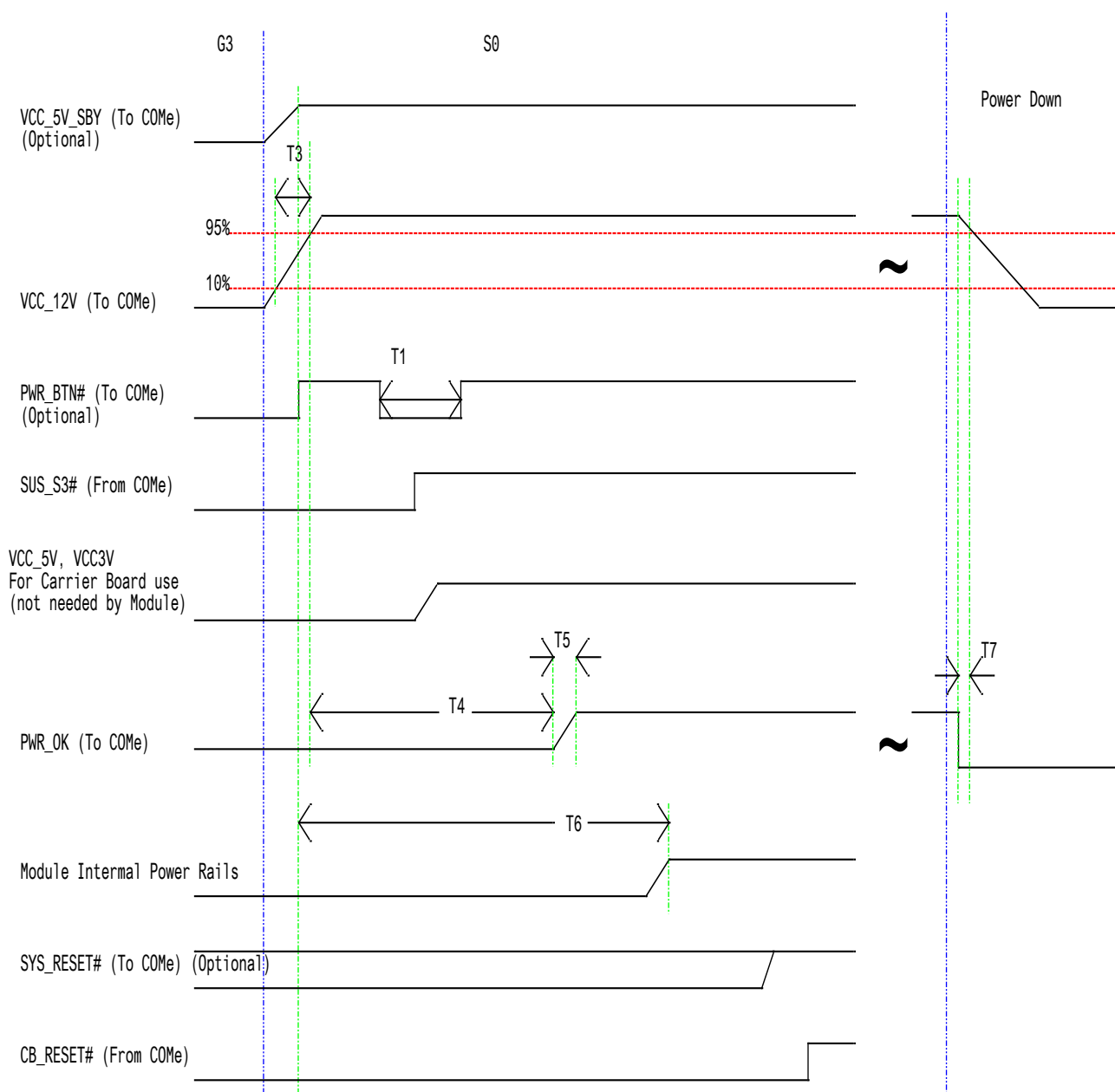
Figure 22: AT Style Power Up Boot
