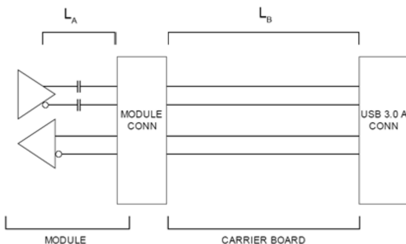
Figure 13: Topology for USB3.0
