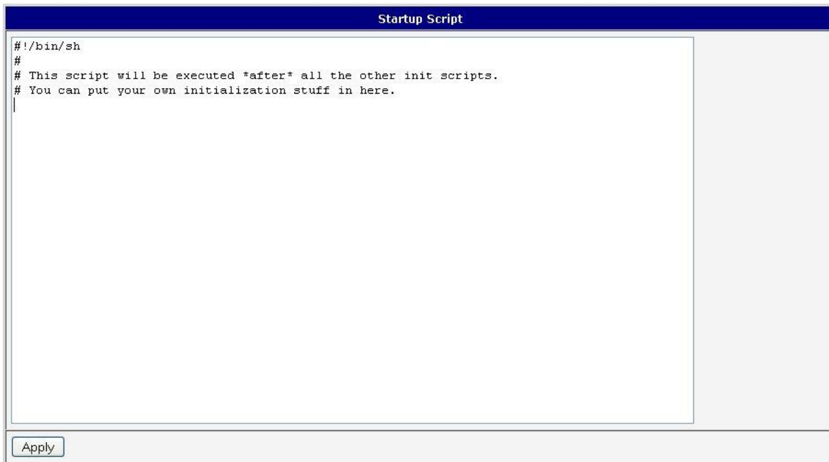
Figure 622. Startup script
