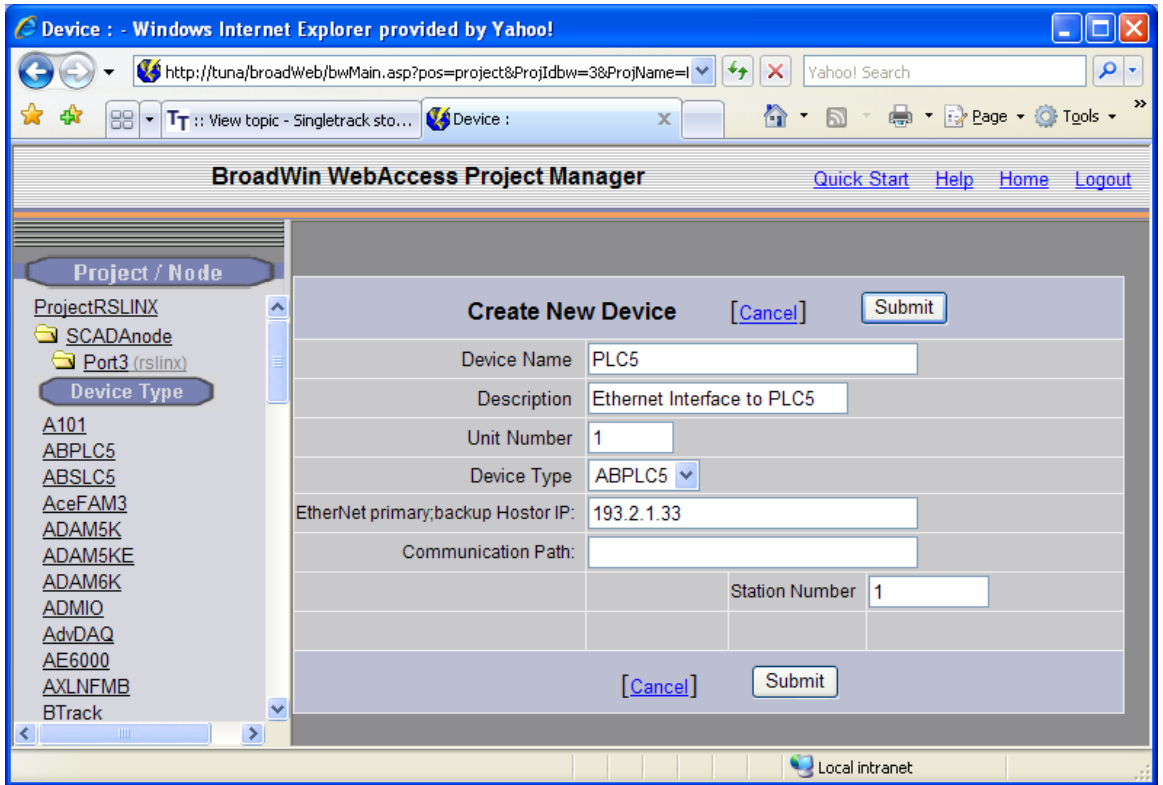
Figure 3-13 Allen-Bradley PLC5 Device on Ethernet Interface (EI) comport
