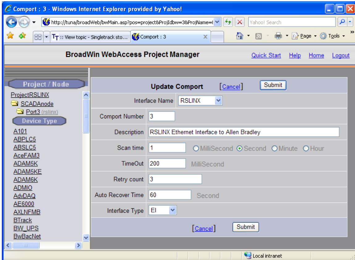
Figure 3.1 RSLINX Comport properties for Ethernet Interface
