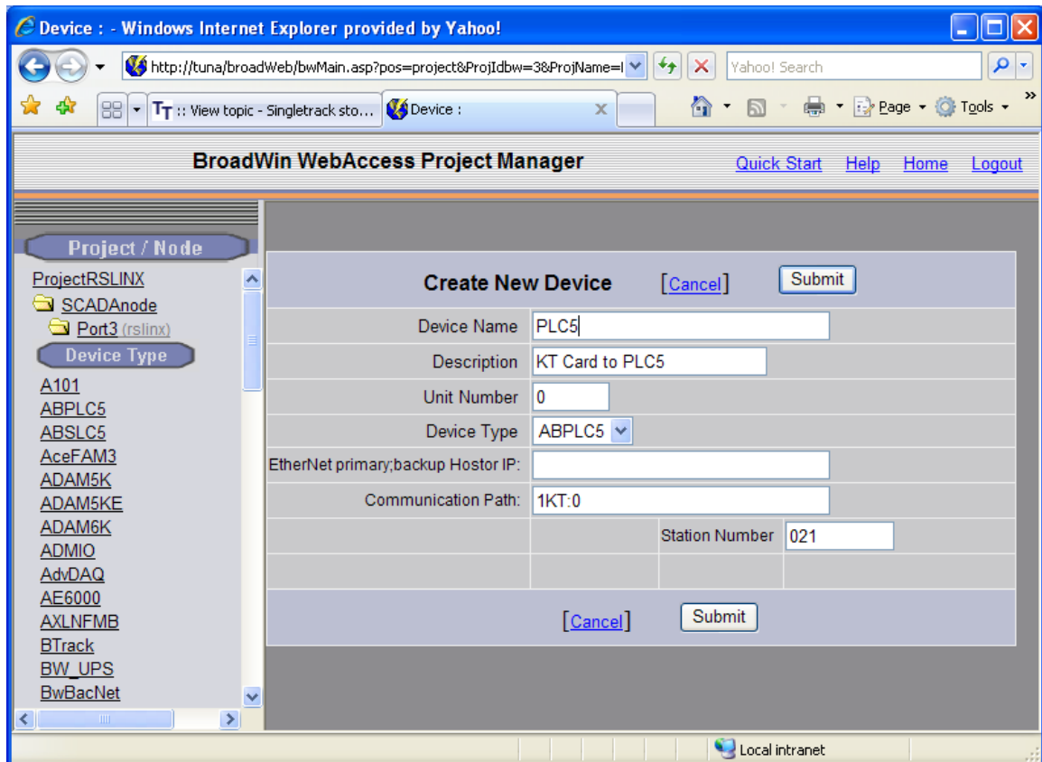
Figure 3-12 Allen-Bradley PLC5 Device on KT type comport
