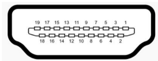
Figure 2.12 HDMI Connector
