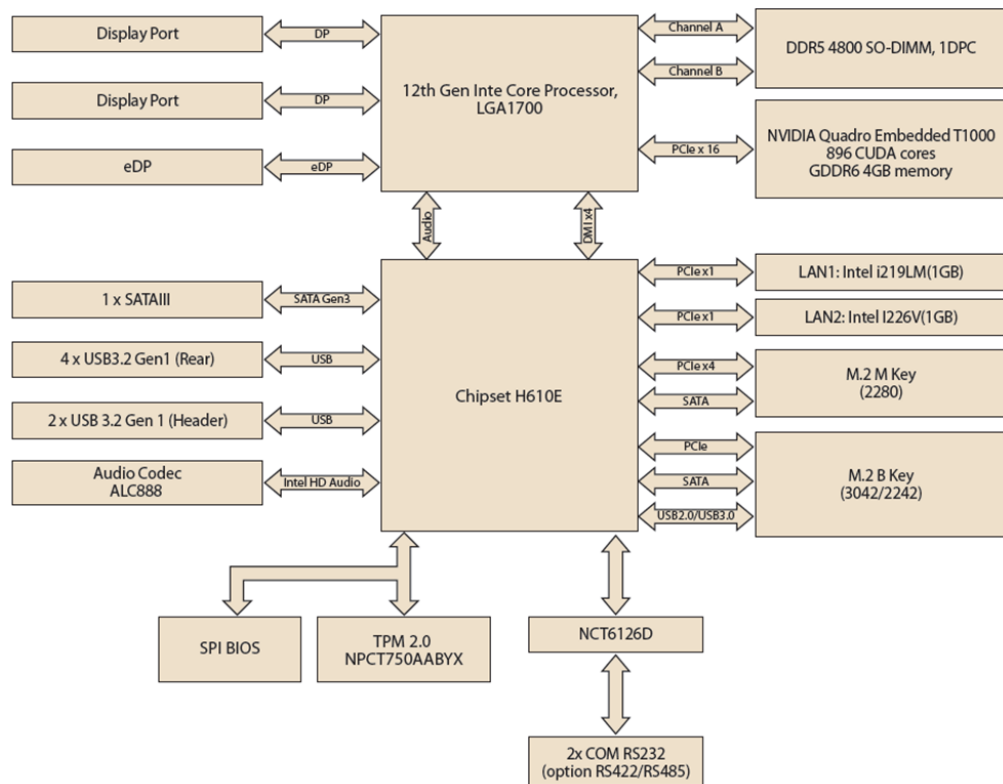
Figure 1.3 AIMB-288E Board Diagram
