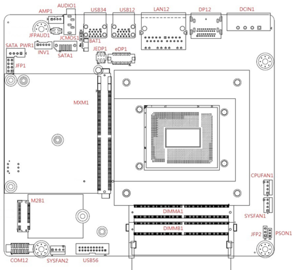
Figure 1.1 Jumper and Connector Locations (Top Side)
