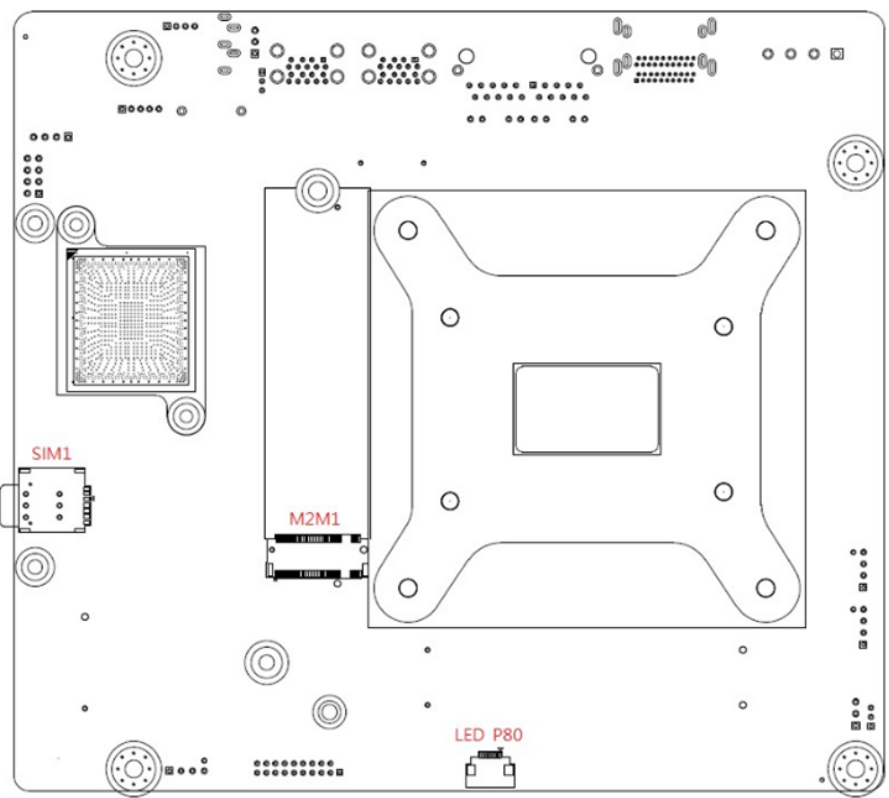
Figure 1.2 Jumper and Connector Locations (Bottom Side)
