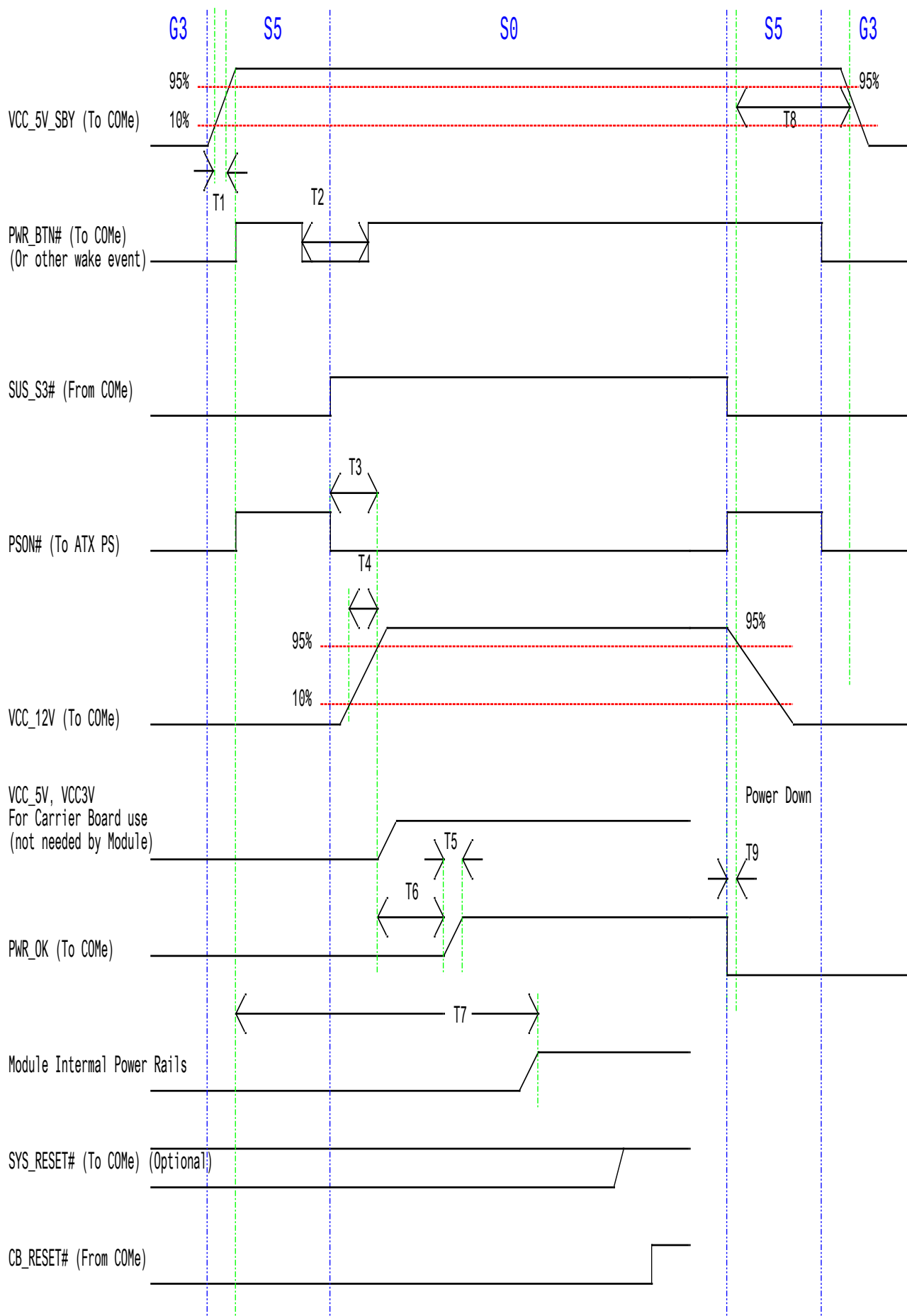
Figure 37: ATX Style Power Up Boot – Controlled by Power Button
