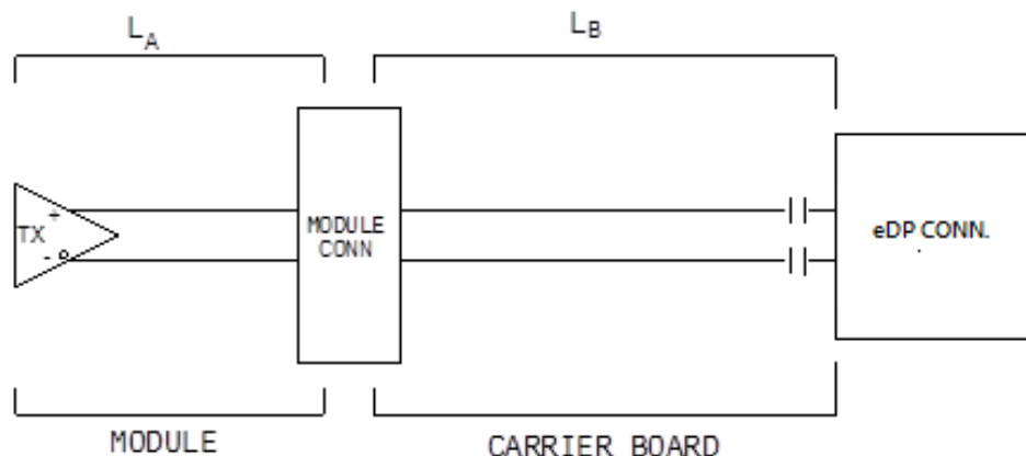
Figure 23: Topology for eDP
