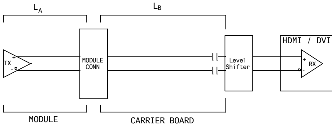
Figure 11: Topology for HDMI / DVI
