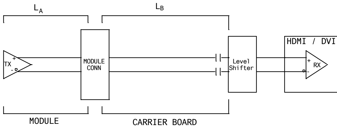
Figure 11: Topology for HDMI / DVI
