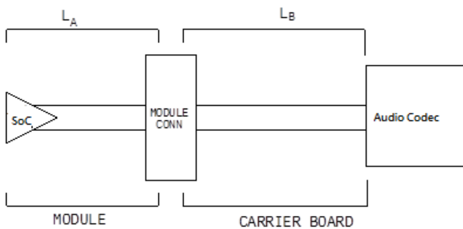
Figure 25: Topology for Audio
