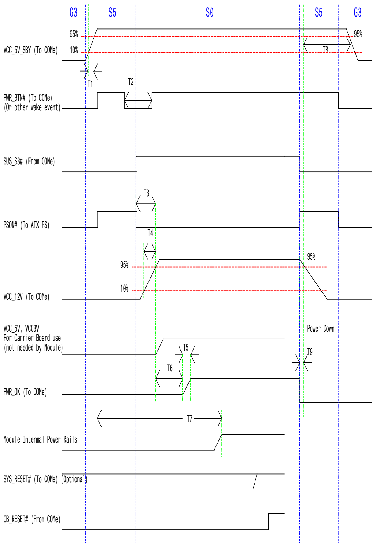
Figure 37: ATX Style Power Up Boot – Controlled by Power Button
