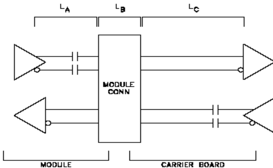
Figure 7: Topology for PCI Express Device Down.
