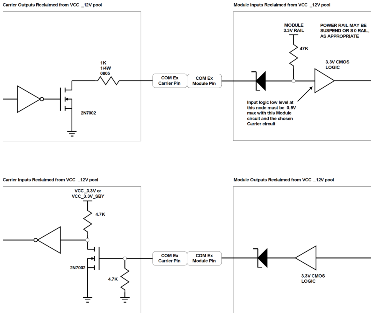
Figure 35: Protecting Logic Level Signals on Pins Reclaimed from VCC_12V
