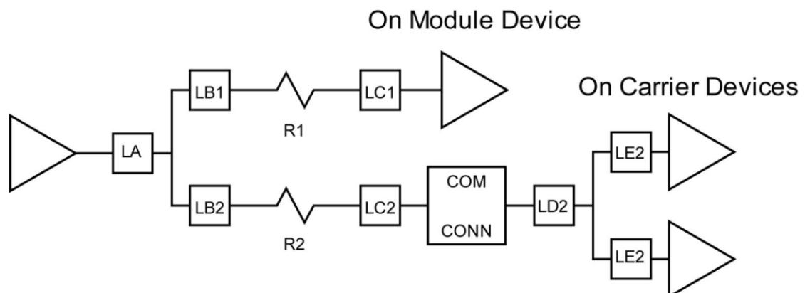
Figure 26: Typical Routing Topology for a Module LPC Device
