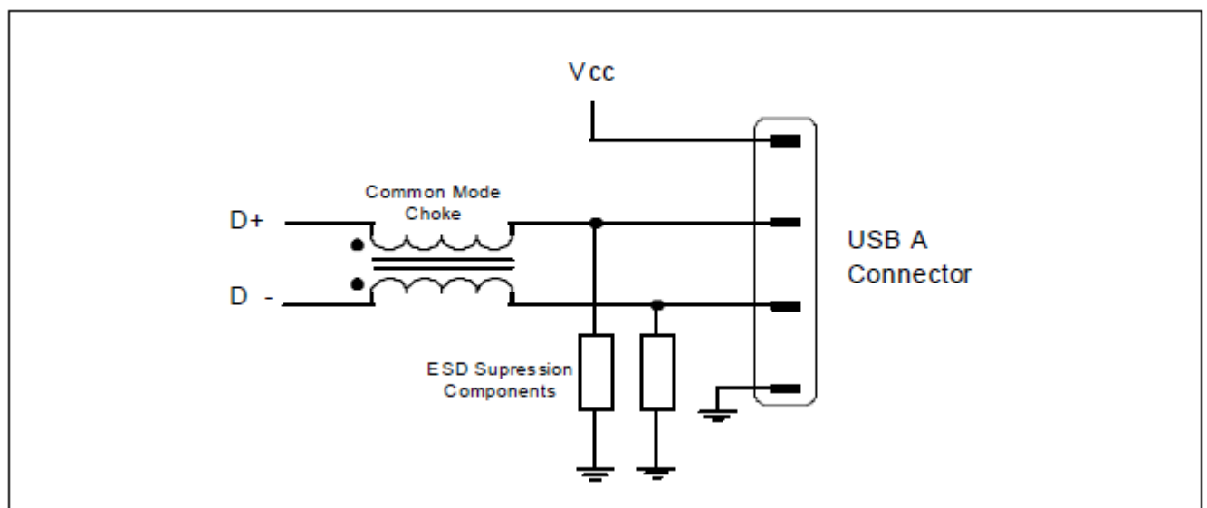
Figure 16: USB 2.0 A Common Mode Choke
