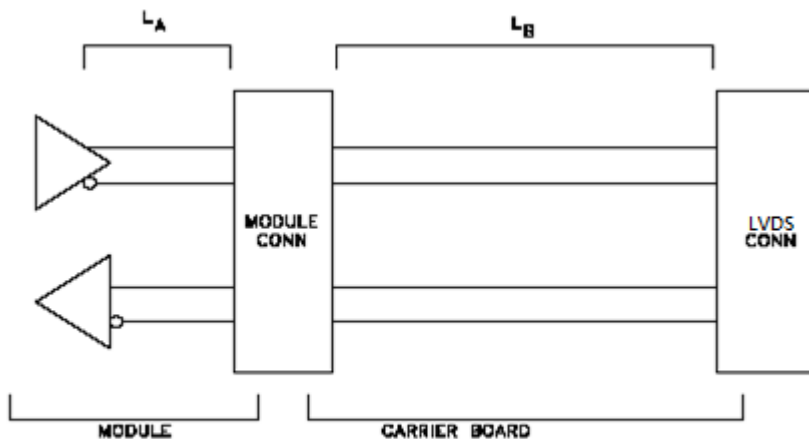
Figure 22: Topology for LVDS
