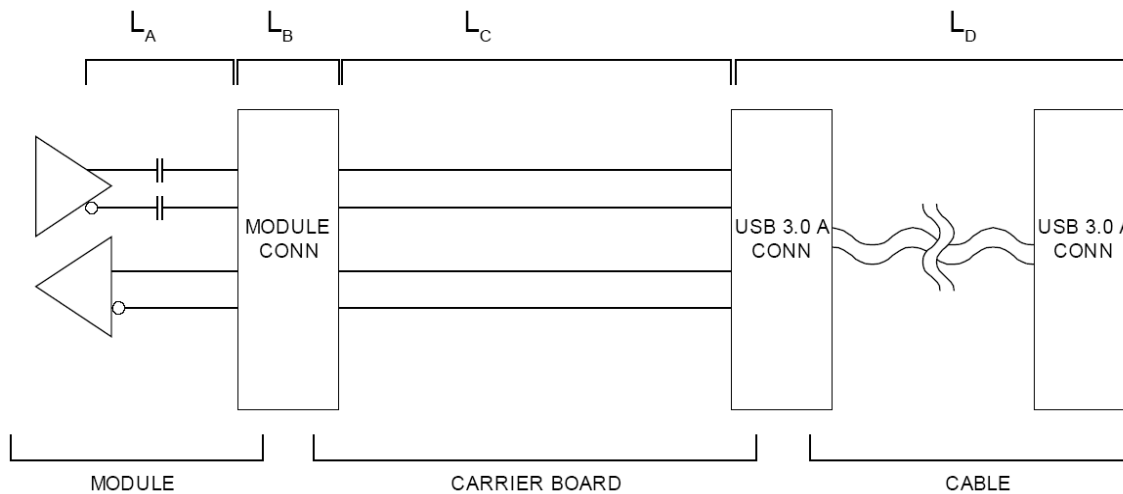
Figure 18: USB3.0/USB3.2 Insertion Loss Budget
