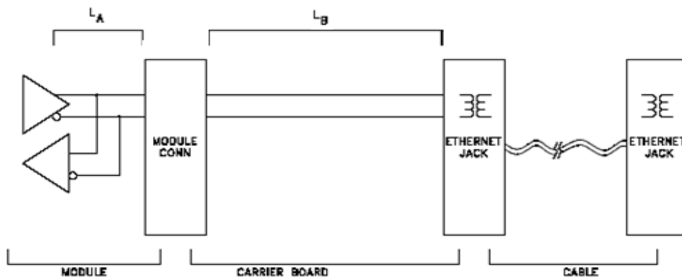
Figure 13: Topology for Ethernet Jack
