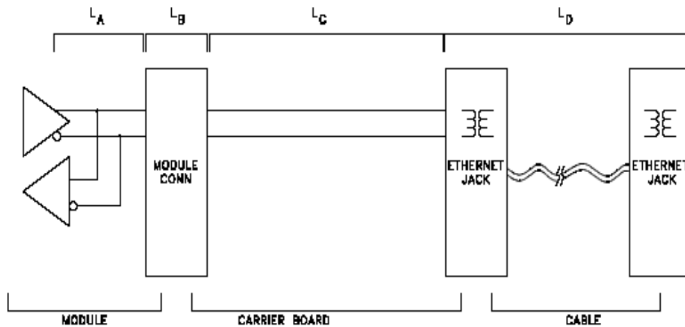
Figure 12: 10/100/1000 Ethernet Insertion Loss Budget
