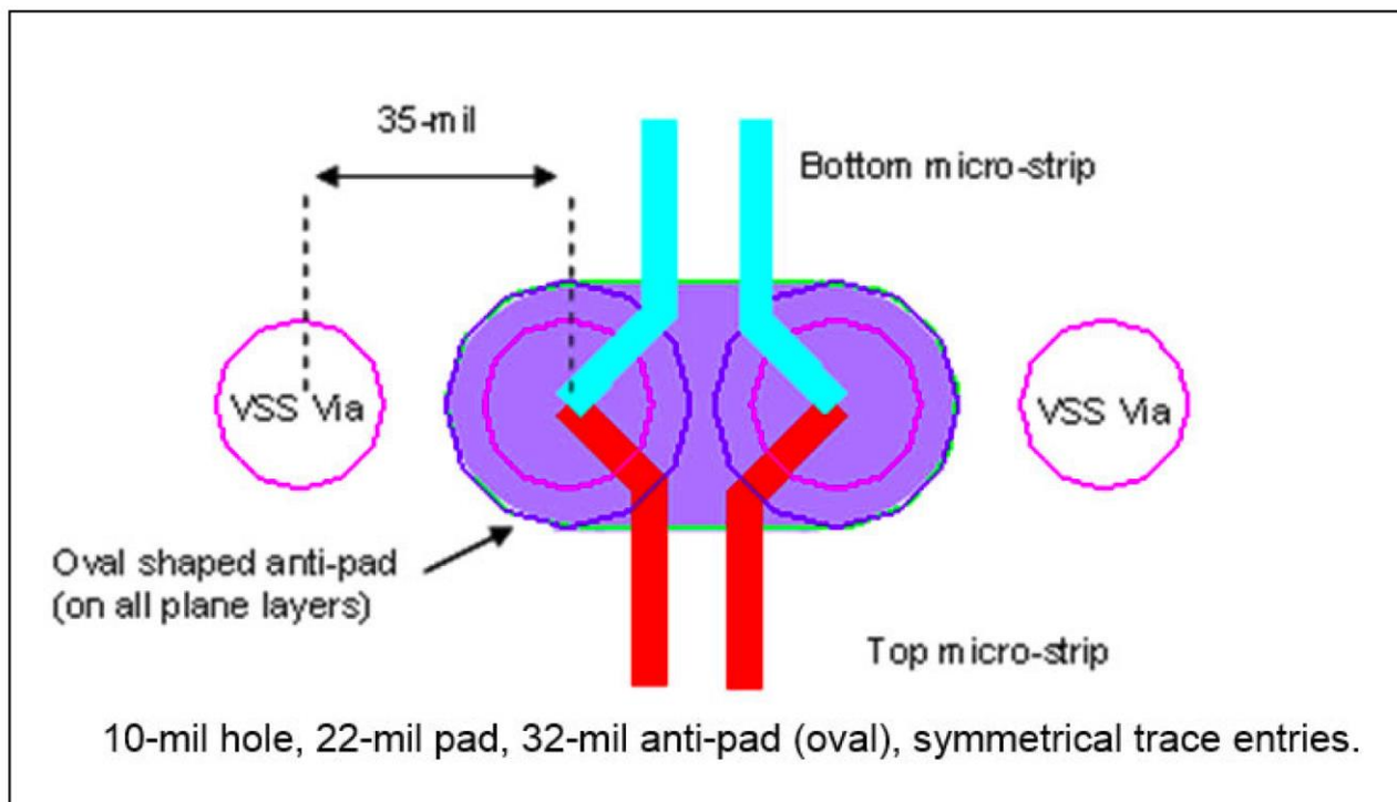
Figure 3: Differential Transitional Via Layout
