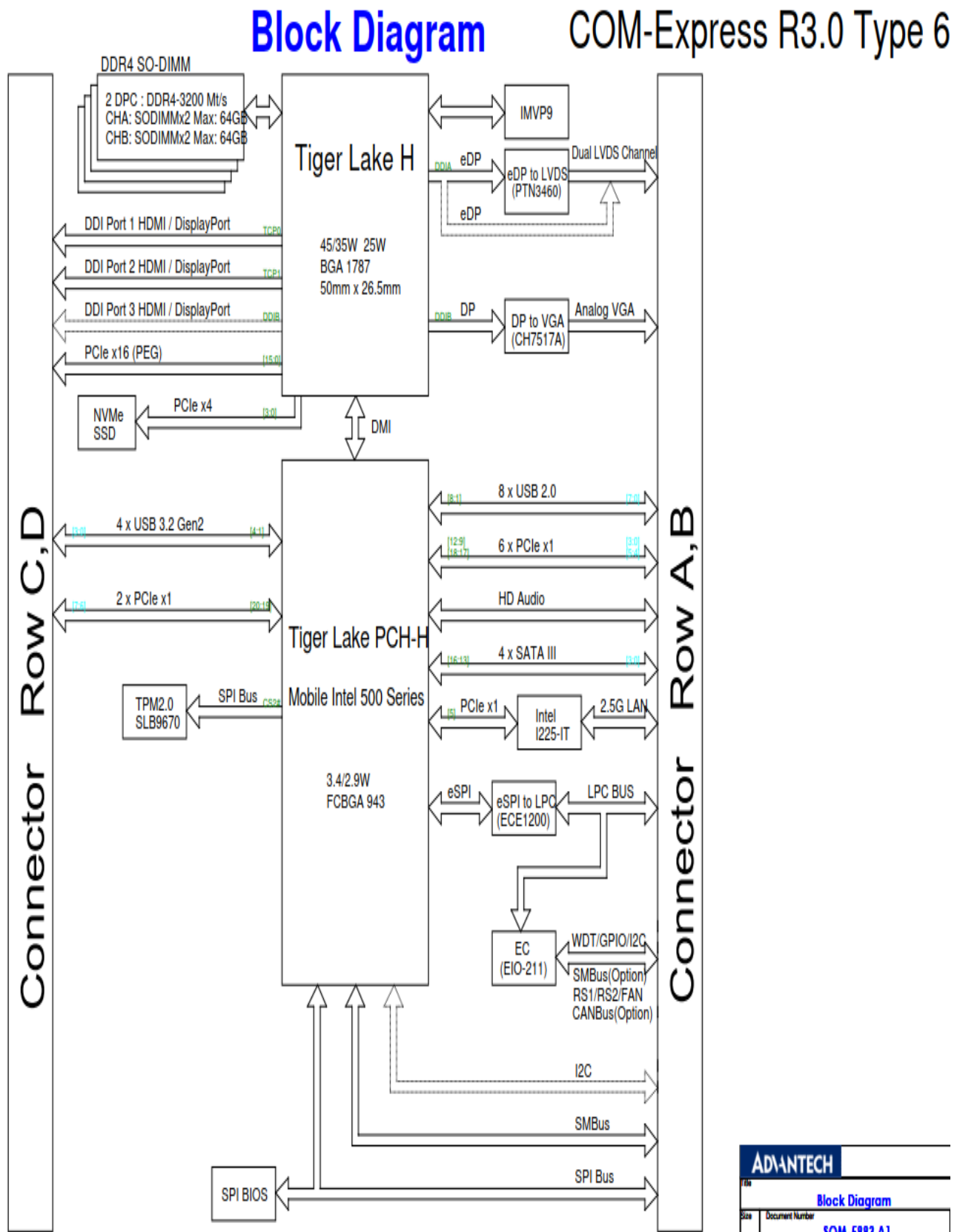
Figure 1: SOM-5883 Block Diagram
