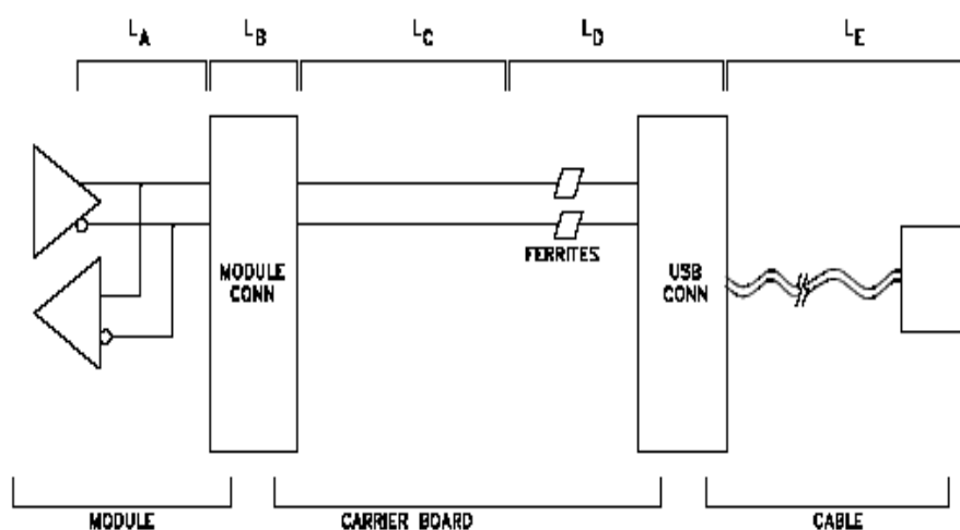
Figure 14: USB2.0 Insertion Loss Budget
