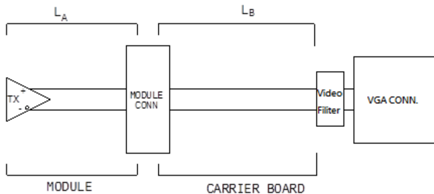
Figure 24: Topology for VGA
