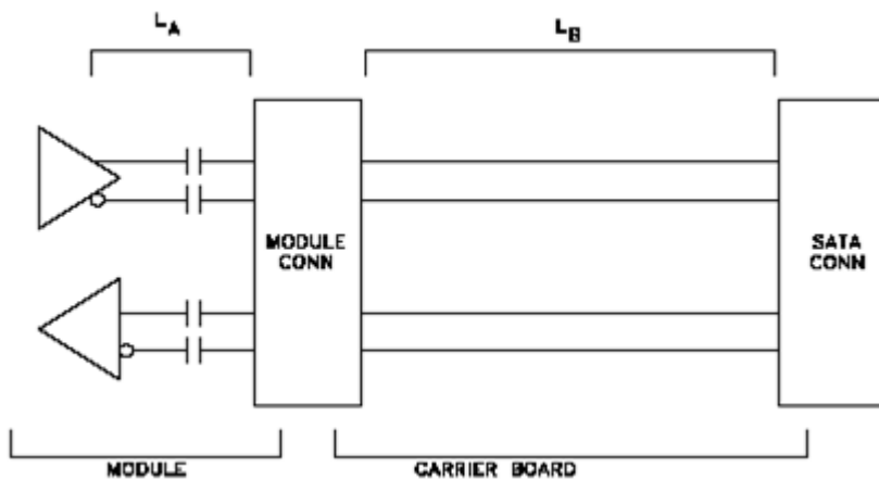
Figure 21: Topology for SATA
