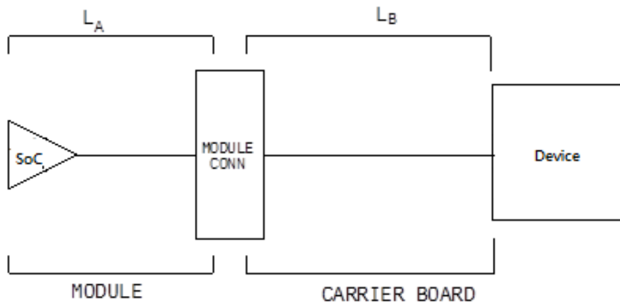
Figure 36: Topology for SDIO
