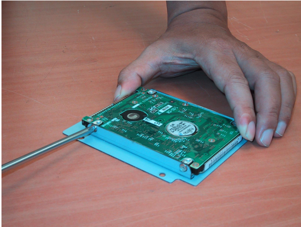
Figure 3-1: Install the HDD on the HDD bracket
