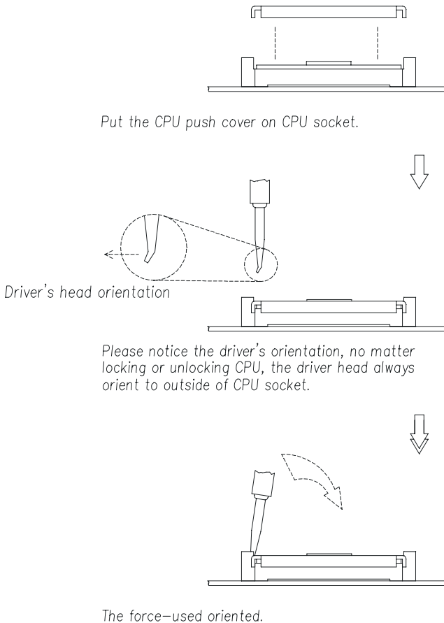
Figure 3-7: CPU installation
