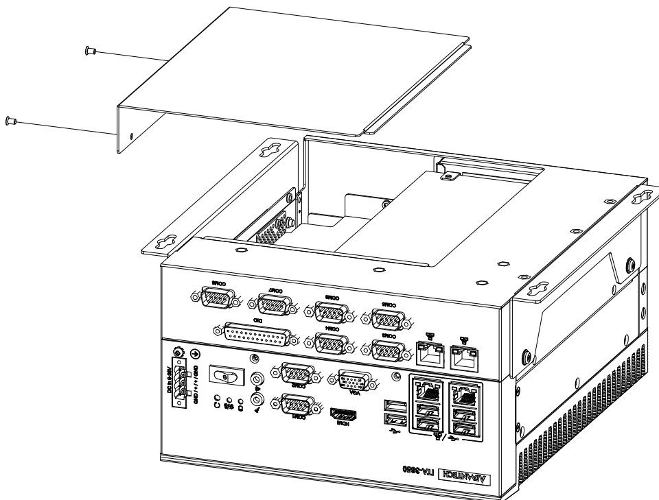
Figure 3.4 Installing the Top Cover
