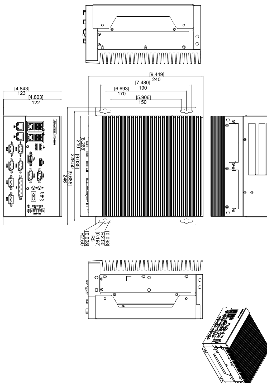
Figure 1.1 Dimension Diagram of ITA-3650E
