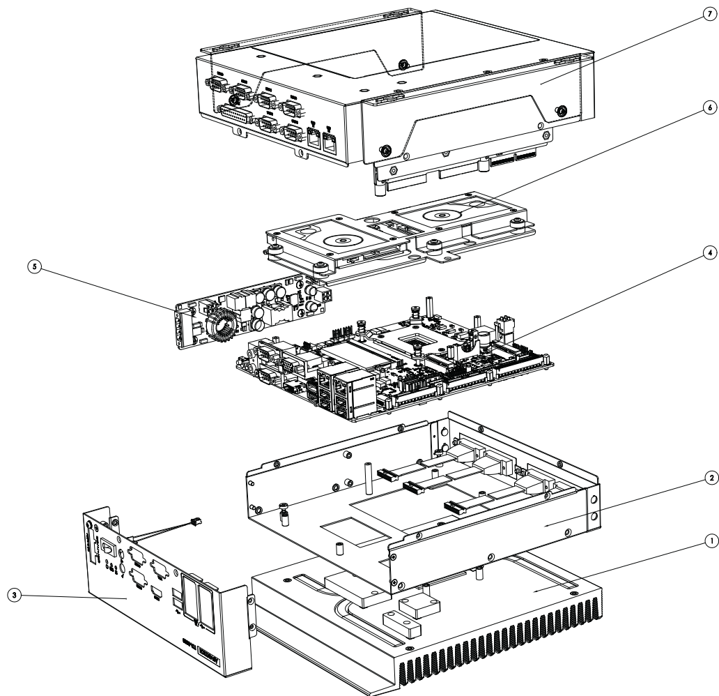
Figure 1.2 Exploded Diagram of ITA-3650E
