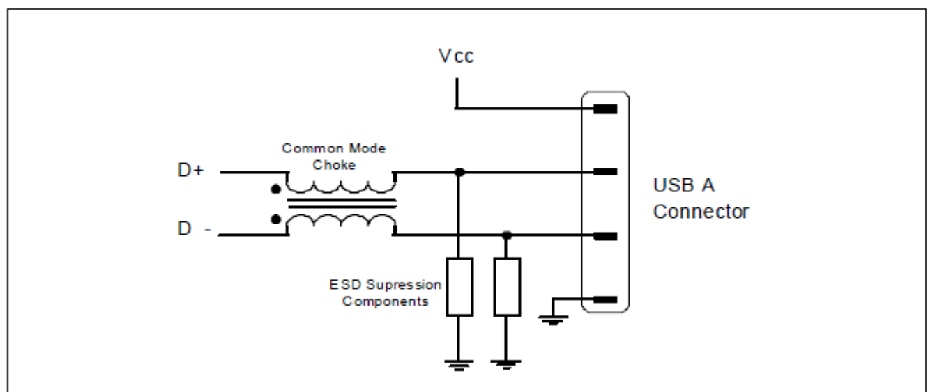
Figure 13: USB 2.0 A Common Mode Choke
