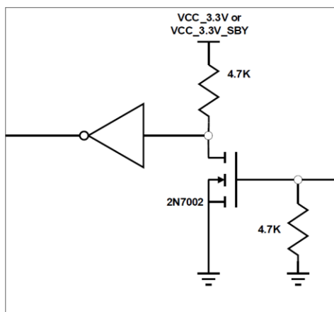
Carrier Inputs Reclaimed from VCC _12V pool
