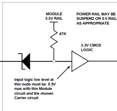
Module Inputs Reclaimed from VCC _12V pool
