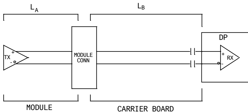
Figure 9: Topology for DisplayPort
