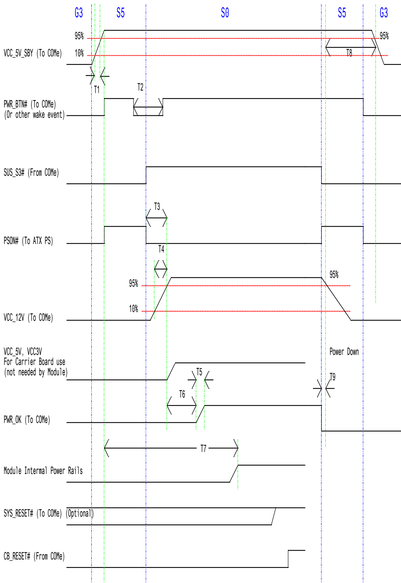
Figure 42: AT Style Power Up Boot
