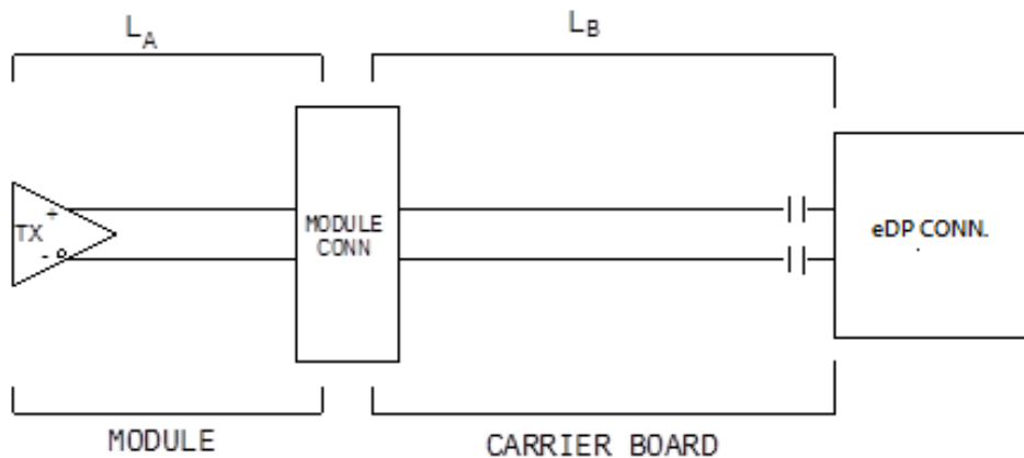
Figure 23: Topology for eDP
