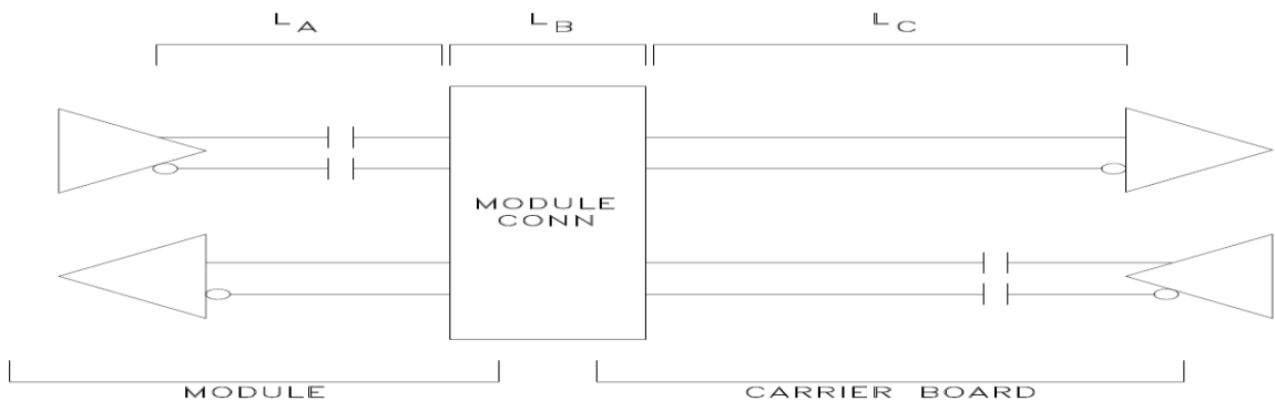
Figure 2: PCI Express Insertion Loss Budget with Carrier Board PCIe Device
