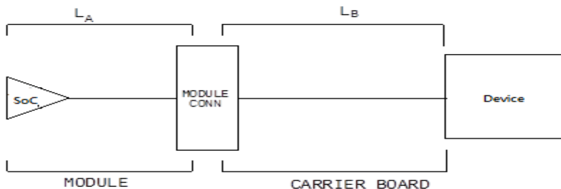
Figure 34: Topology for CAN interface
