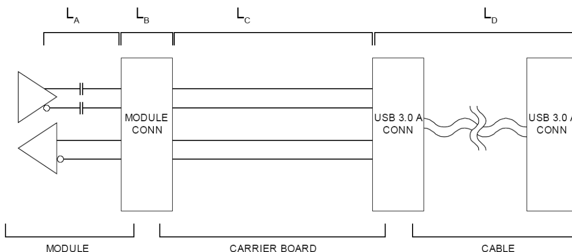
Figure 18: USB3.0/USB3.2 Insertion Loss Budget
