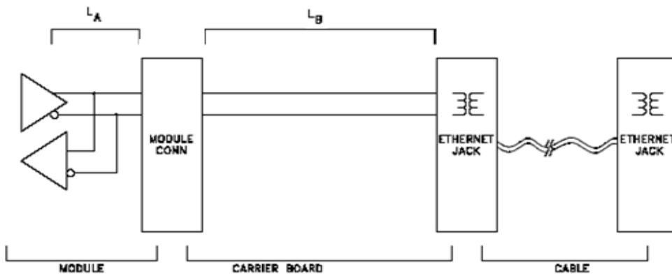
Figure 13: Topology for Ethernet Jack
