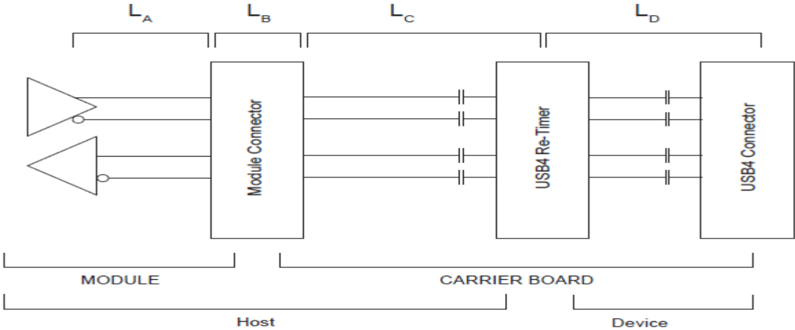
Figure 40: USB4 Insertion Loss Budget, with Carrier Retimer
