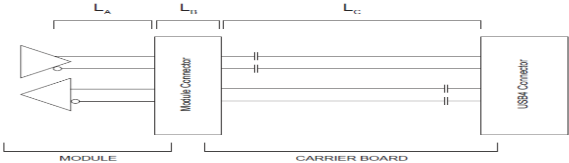
Figure 39: USB4 Insertion Loss Budget, without Carrier Retimer
