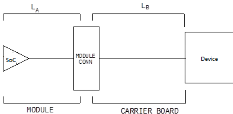
Figure 25: Topology for LPC
