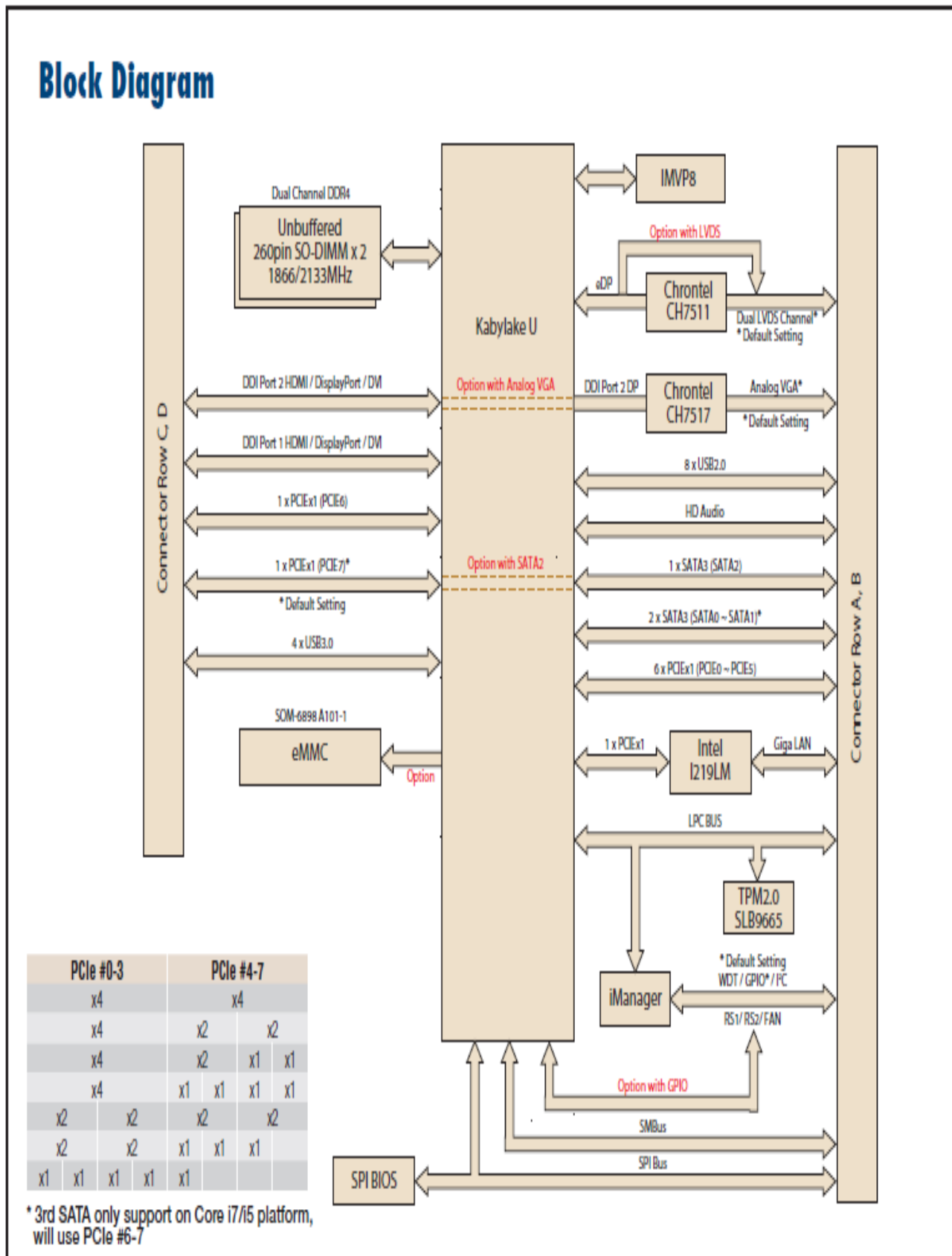
Figure 1: SOM-6889 Block Diagram
