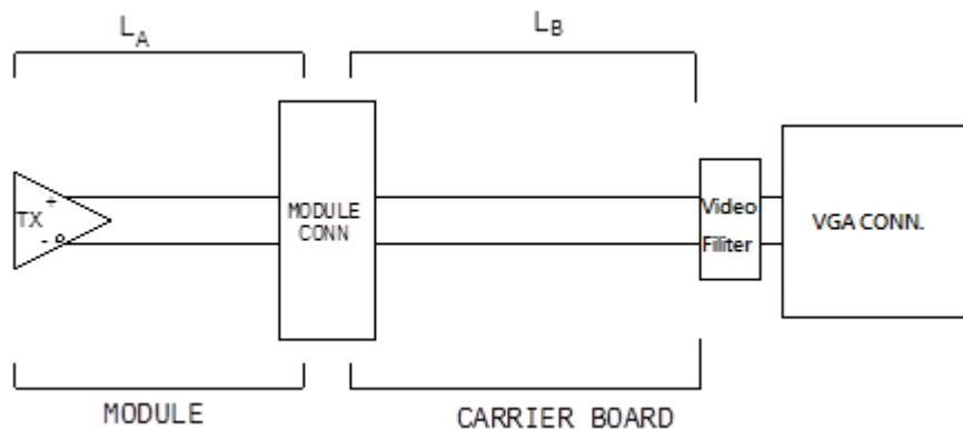
Figure 23: Topology for VGA
