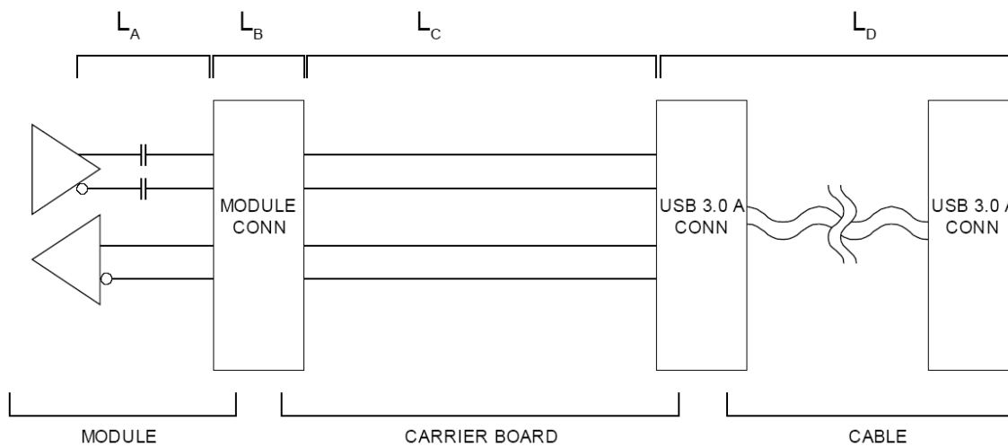
Figure 17: USB3.0 Insertion Loss Budget
