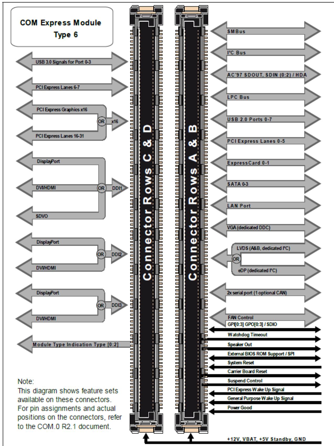
Figure 2: COM Express Type6 Connector Layout
