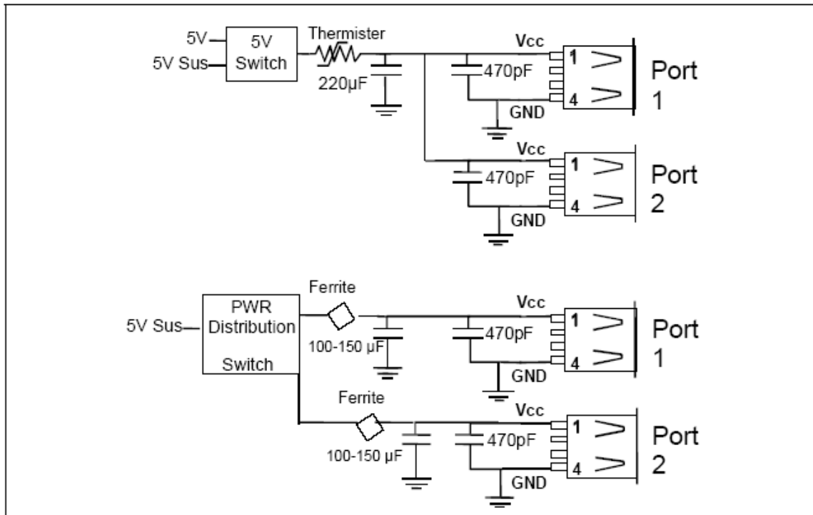
Figure 14: USB 2.0 Good Downstream Power Connection
