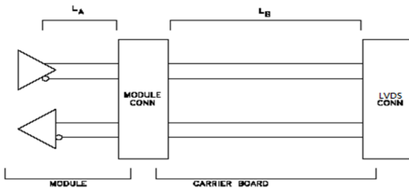
Figure 21: Topology for LVDS
