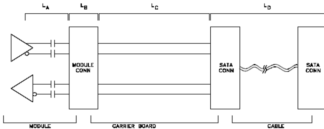
Figure 19: SATA Insertion Loss Budge
