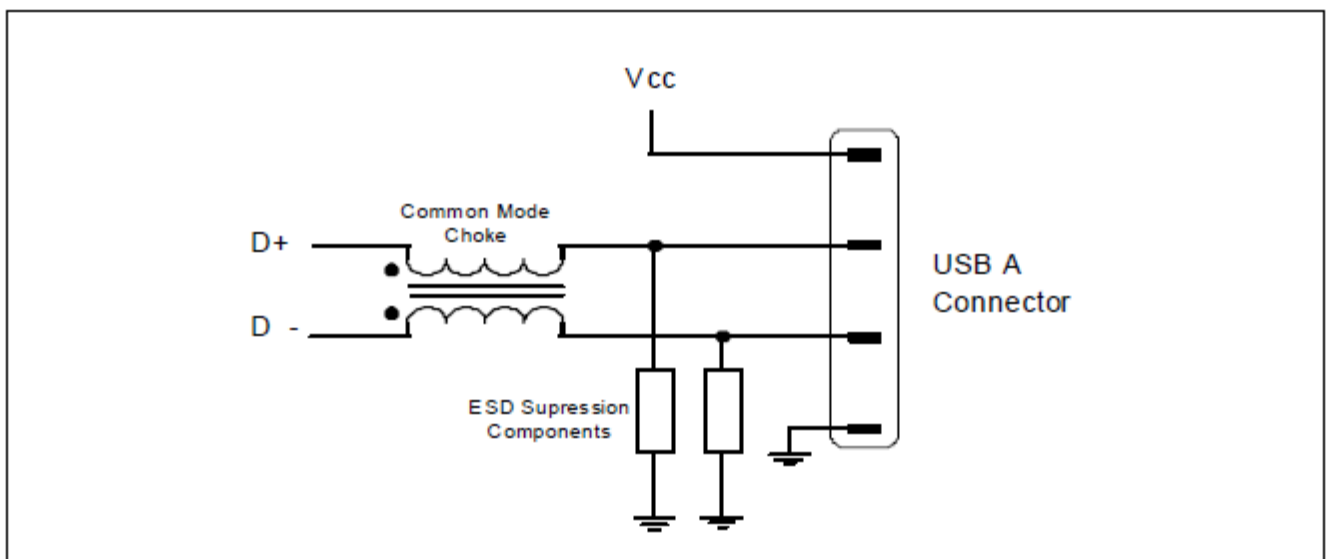
Figure 15: USB 2.0 A Common Mode Choke
