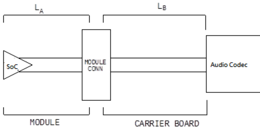
Figure 24: Topology for Audio
