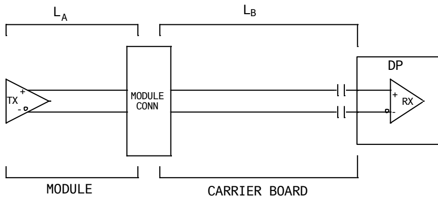
Figure 8: Topology for DisplayPort
