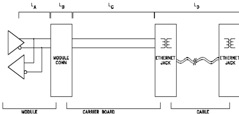
Figure 11: 10/100/1000 Ethernet Insertion Loss Budget
