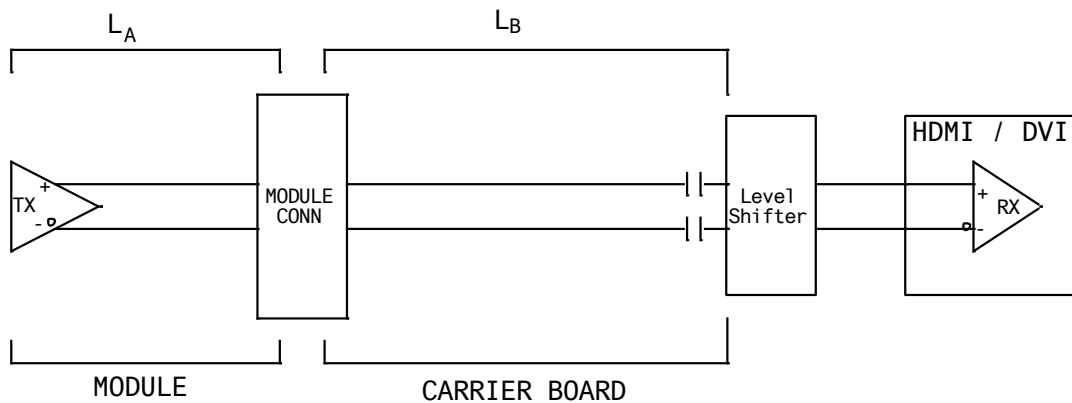
Figure 10: Topology for HDMI / DVI
