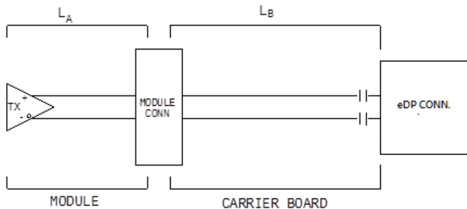
Figure 22: Topology for eDP
