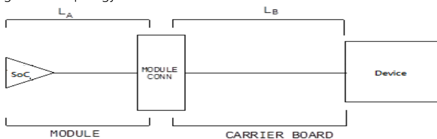
Figure 26: Topology for LPC
