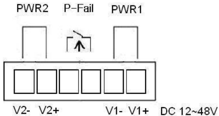
Figure 2.6-1 Power Connector
