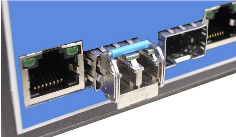
Figure 2.5-2 Transceiver inserted
