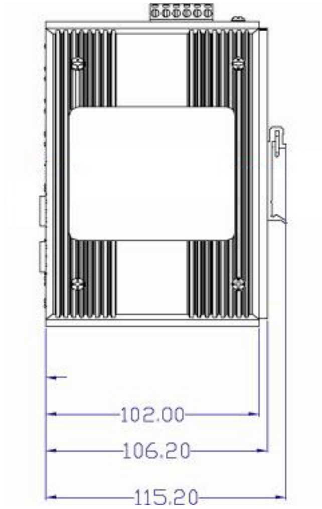
Figure 2.2-2 Side View
