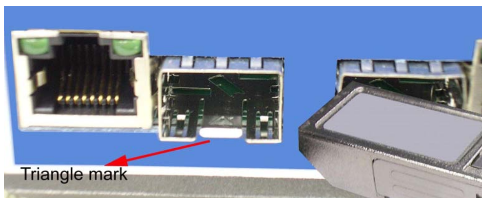
Figure 2.5-1 Transceiver to the SFP slot
