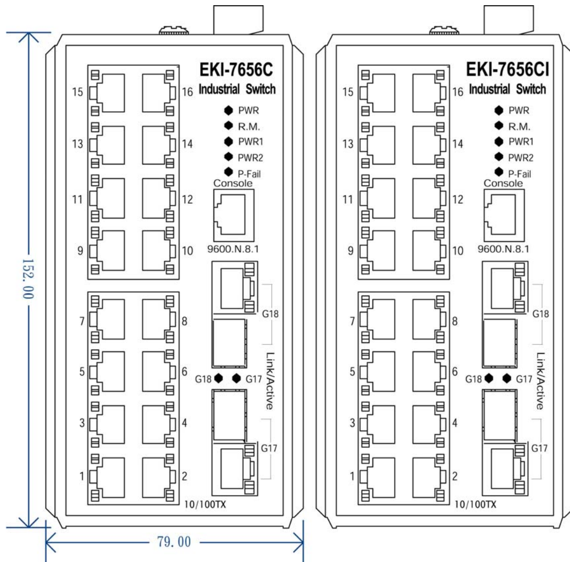
Figure 2.2-1 Front View
