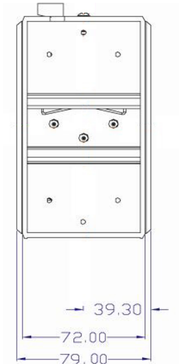
Figure 2.2-3 Rear View
