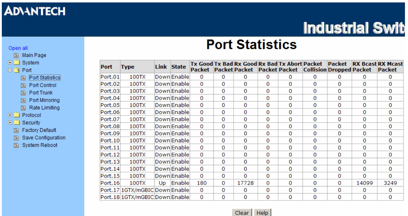
Figure 3.3-19 Port Statistics
