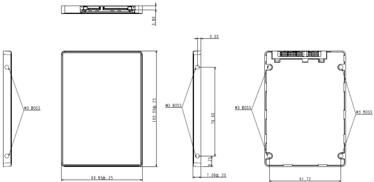
Figure 9-1 Physical Dimensions
