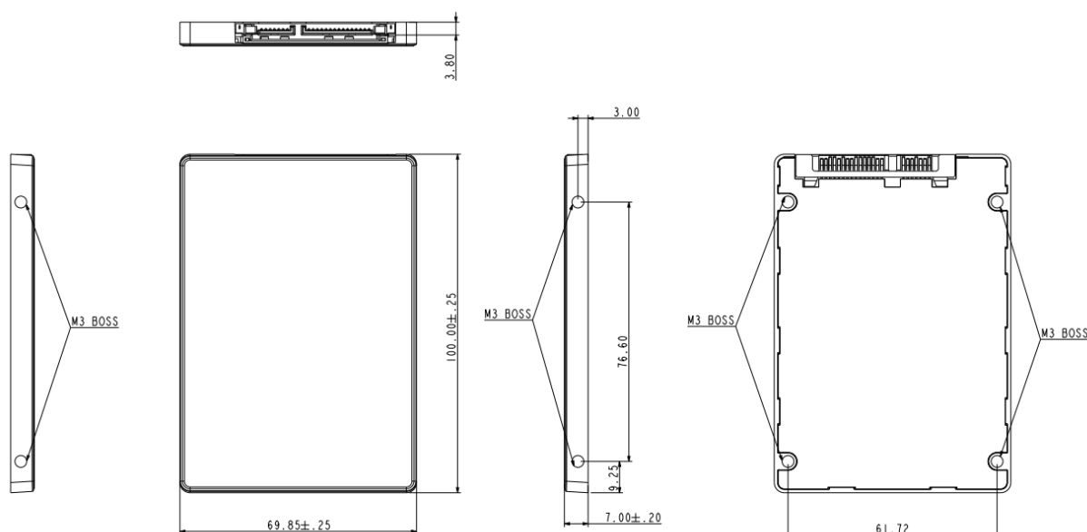
Figure 9-1 Physical Dimensions
