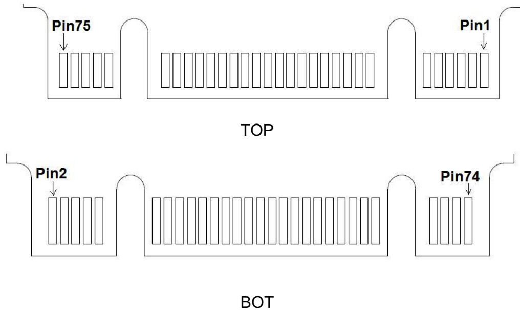
Figure 5-1 SATA Interface
