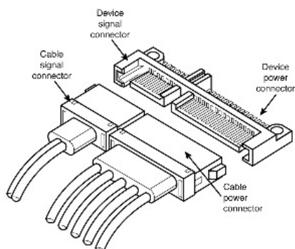
Figure 2 Attaching SATA cabling
