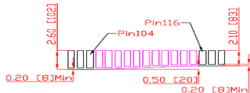
Detail D
