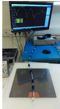
300mm x 300mm Ground Plane Edge
