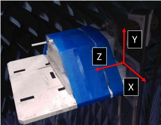
Chamber Setup
