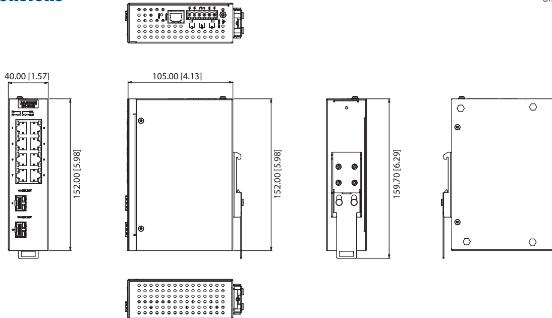
Panel Cut-out Dimensions (W x H x D): 40 x 152 x 105 mm (1.57 x 5.98 x 4.13 inch)
