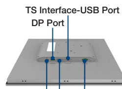
HDMI Port 24V DC Power Input with Phoenix Jack VGA Port
