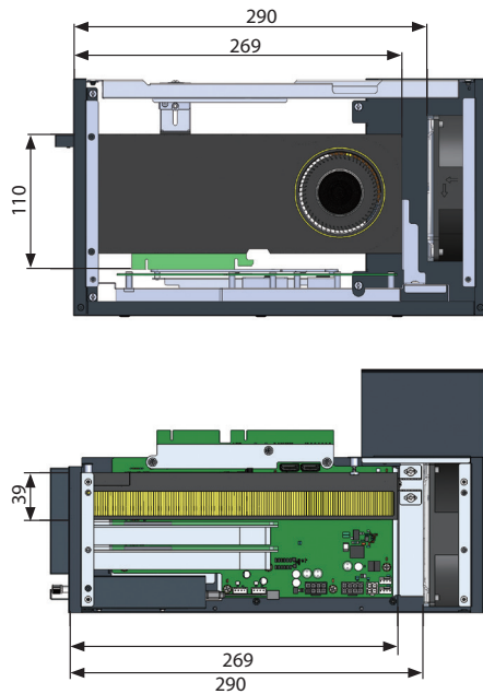
MIC-78MG30 GPU Dimension Guide
