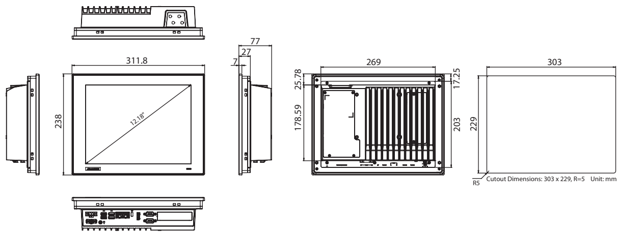
Panel Cut-out Dimensions: 303 x 229 mm (11.93 x 9.02 in)
