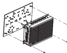
VESA Mount (Optional)
