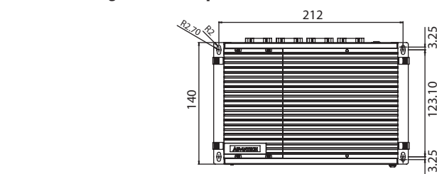
UNO-2484V3 Single stack + Expansion stack
