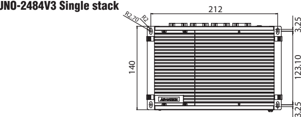
UNO-2484V3 Single stack
